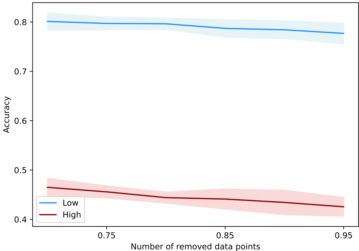
DataAttrOpt(10000, 0.15, 15, best, +b, alpha=best) - imdb-embedding
